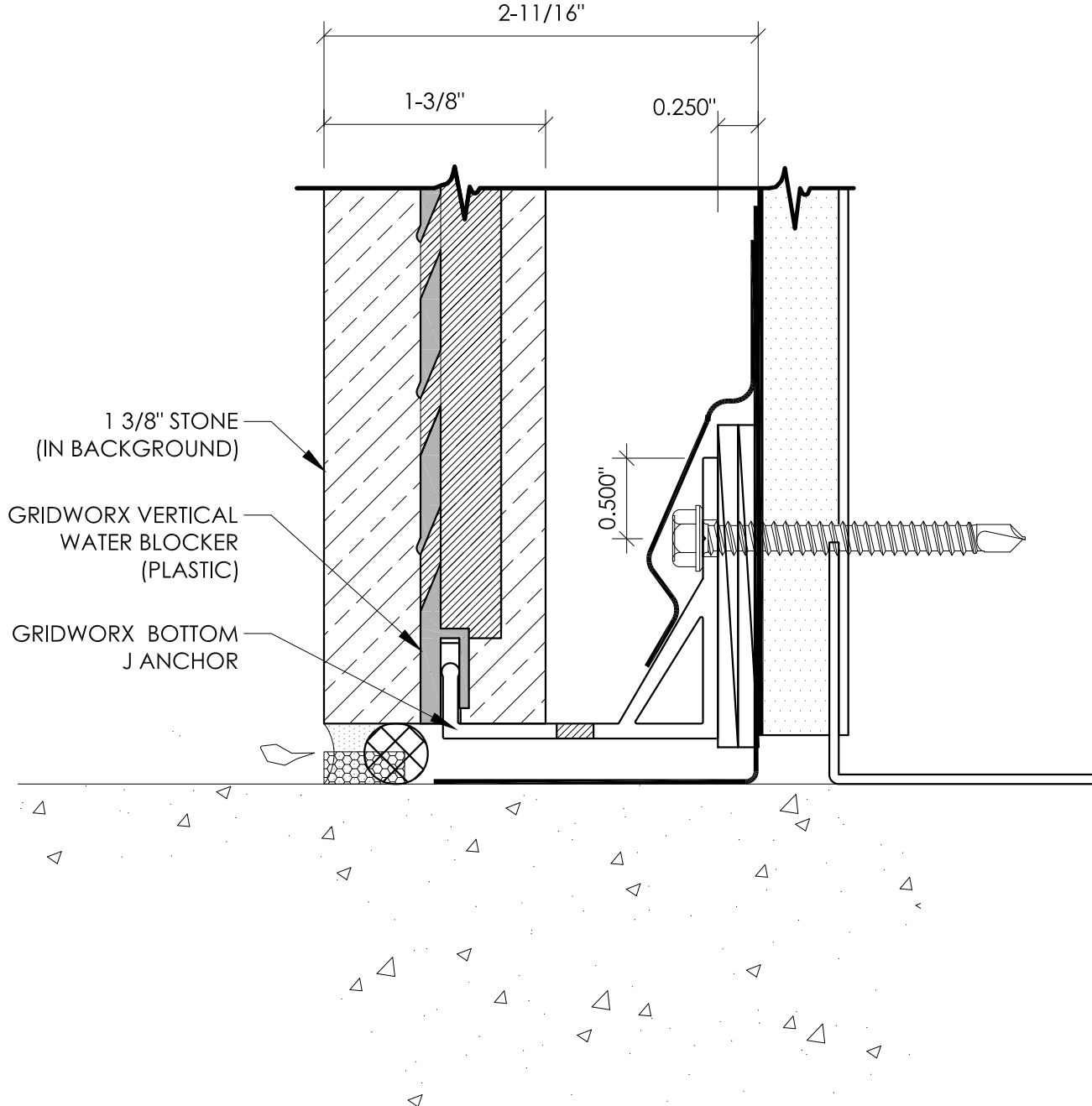
STARTER J ANCHOR SHOWING VERTICAL WATER BLOCKER 3/8" JOINTS - STEEL FRAMING SCALE: FULL
